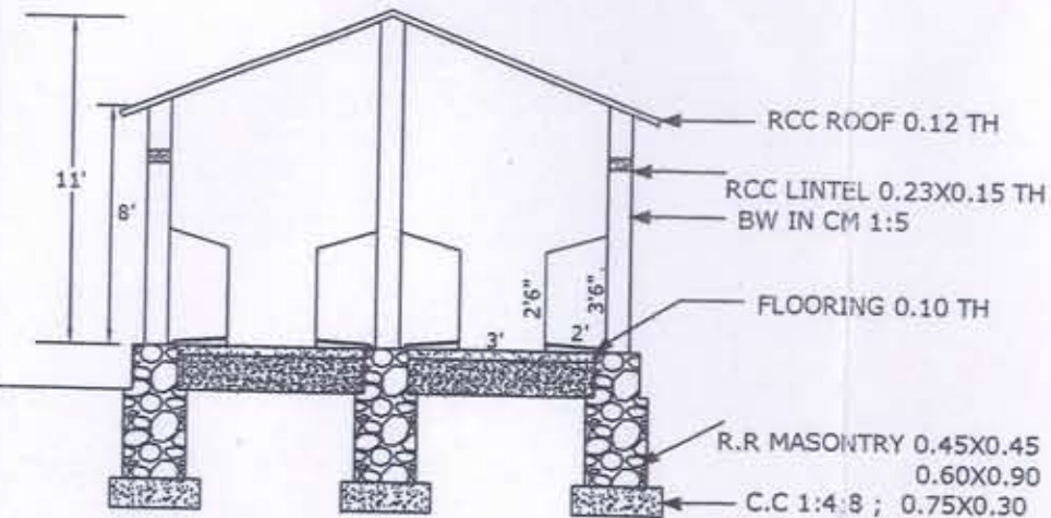
SECTION 'RS'
